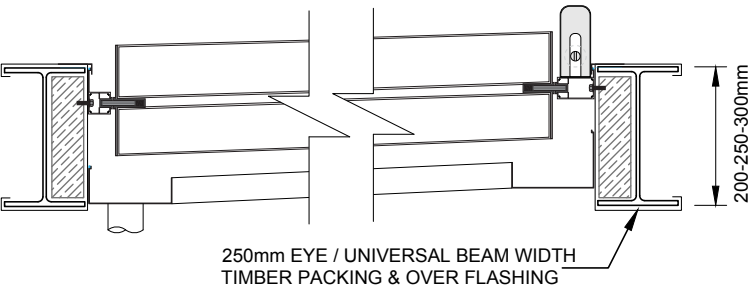
STEEL - EYE BEAM OR UNIVERSIAL
