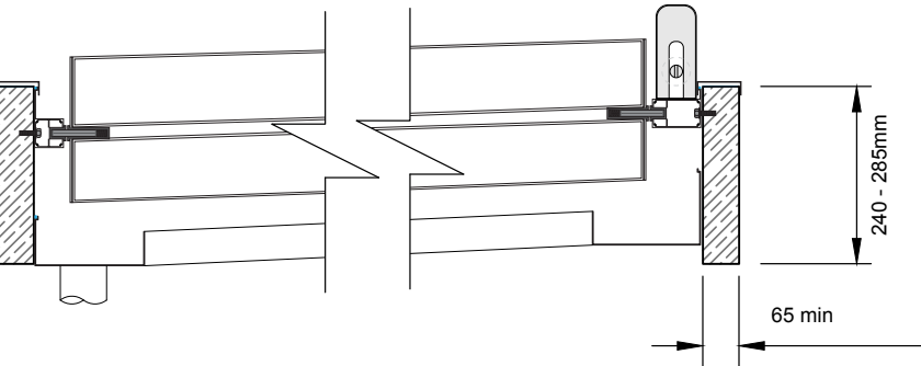
TIMBER - SUPPORT FRAME
