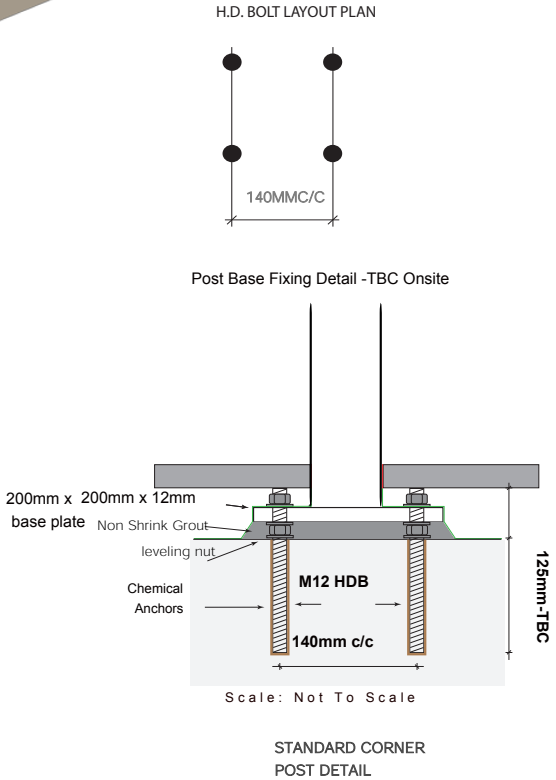
Support Posts
