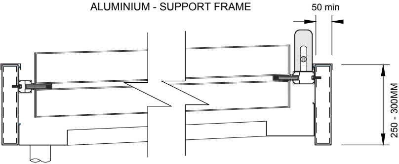
ALUMINIUM - SUPPORT FRAME
