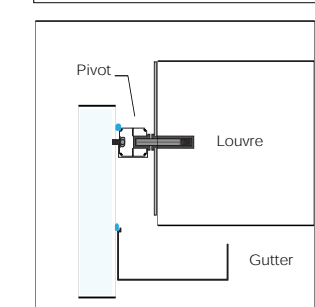
ALUMAX STANDARD DETAIL
